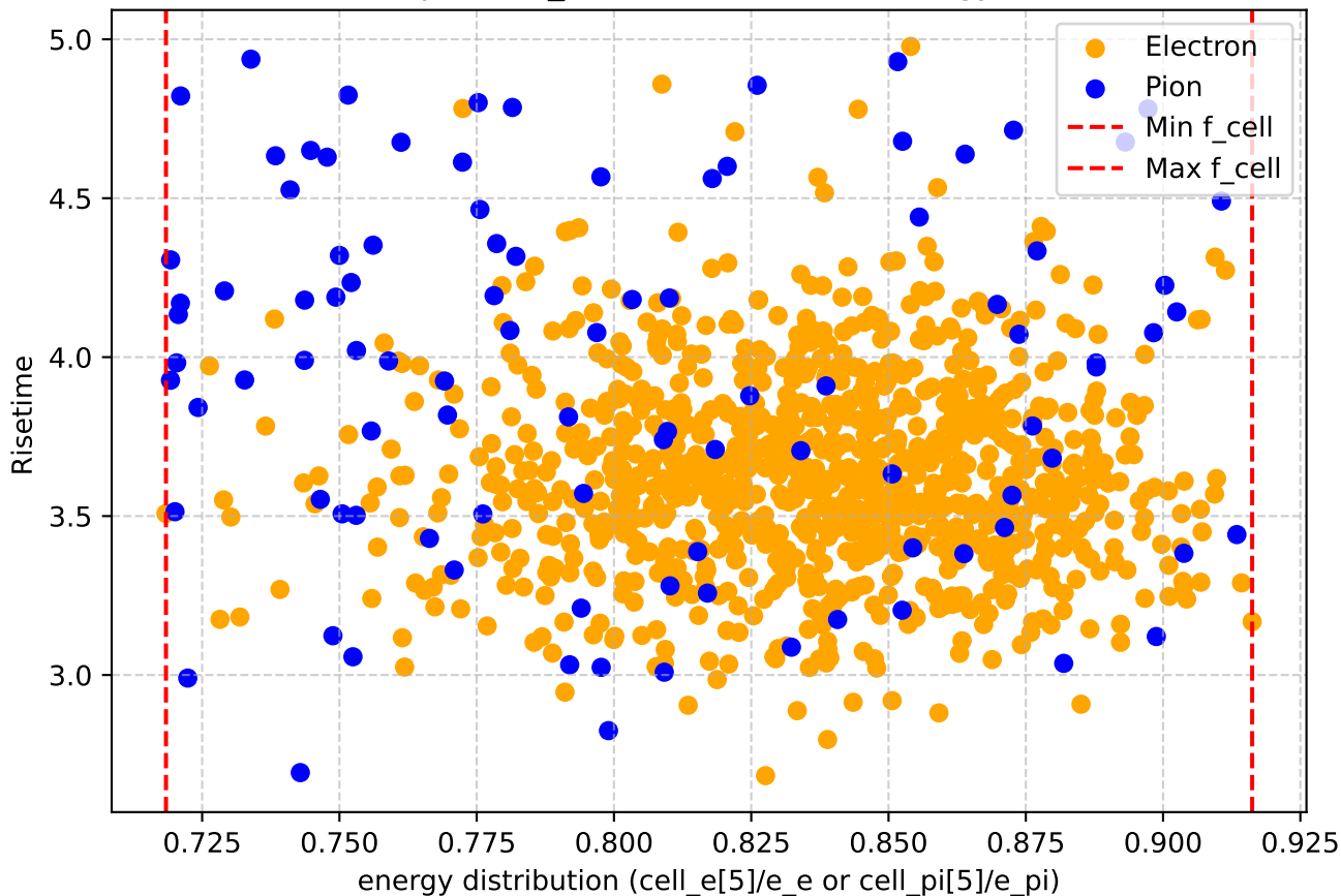
Scatter plot of f_cell vs risetime for energy 2.0GeV
